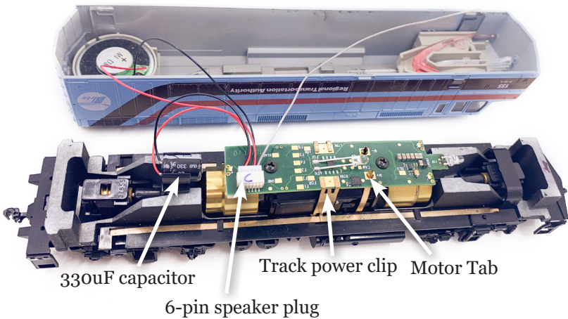
Figure 1: SDXH187K1C: Locomotive with decoder installed
