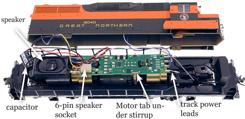
Figure 1: SDXH187Ko: Locomotive with decoder installed
