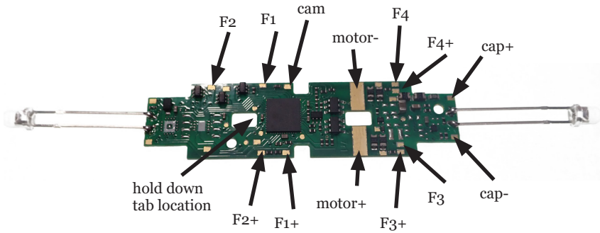
Figure 1: DN167KoA Decoder showing Track/Motor, Function wires,
