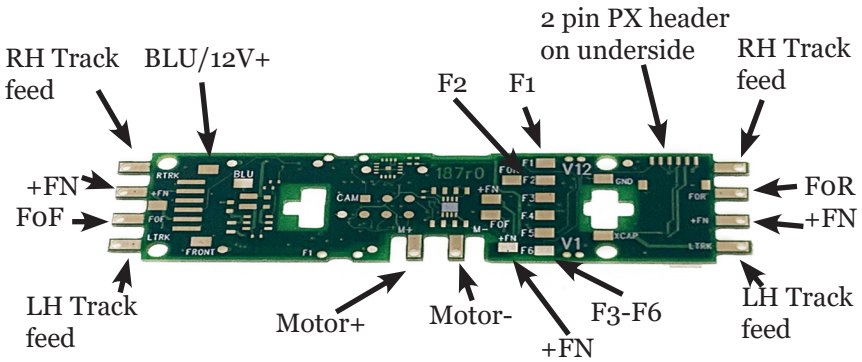
Figure 1: DH187A0:top side connection diagram
