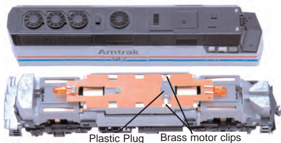
Figure 1: Remove loco shell, remove plastic plug, bend brass motor clips up, slide board forward, remove board
